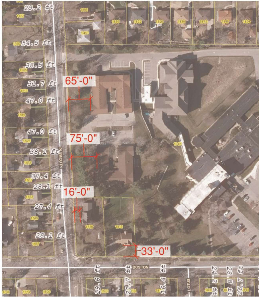
Existing Street Setbacks
